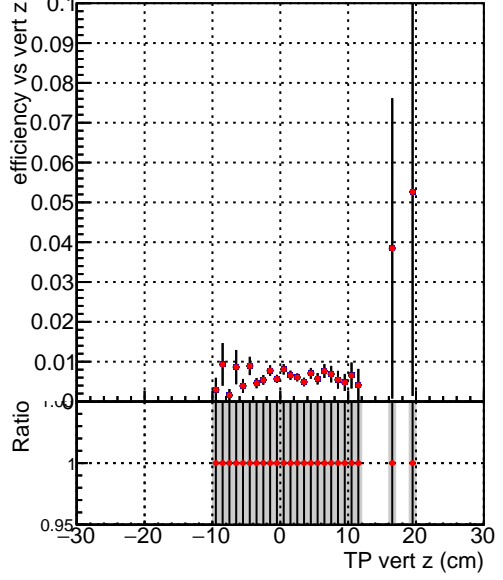
Efficiency vs. TP vert z (cm) — DQM_TT_MKFIT_ORIG — DQM_TT_MKFIT_MODIF
