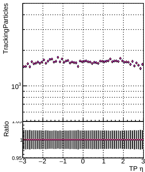
N of sim Model Modif 1 DOM TT MKFITLowPtQ MODIF 2 DOM TT MKFITLowPtT MODIF 3 DOM TT MKFITandPLess MODIF
