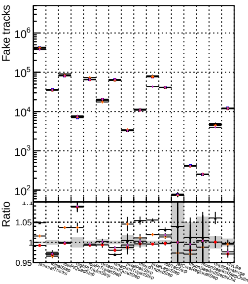
Number Symbol DOM TT MKFITLowPto MODIF DOM TT MKFITLowPto MODIF DOM TT MKFITLowPtt MODIF DOM TT MKFITandPless MODIF
