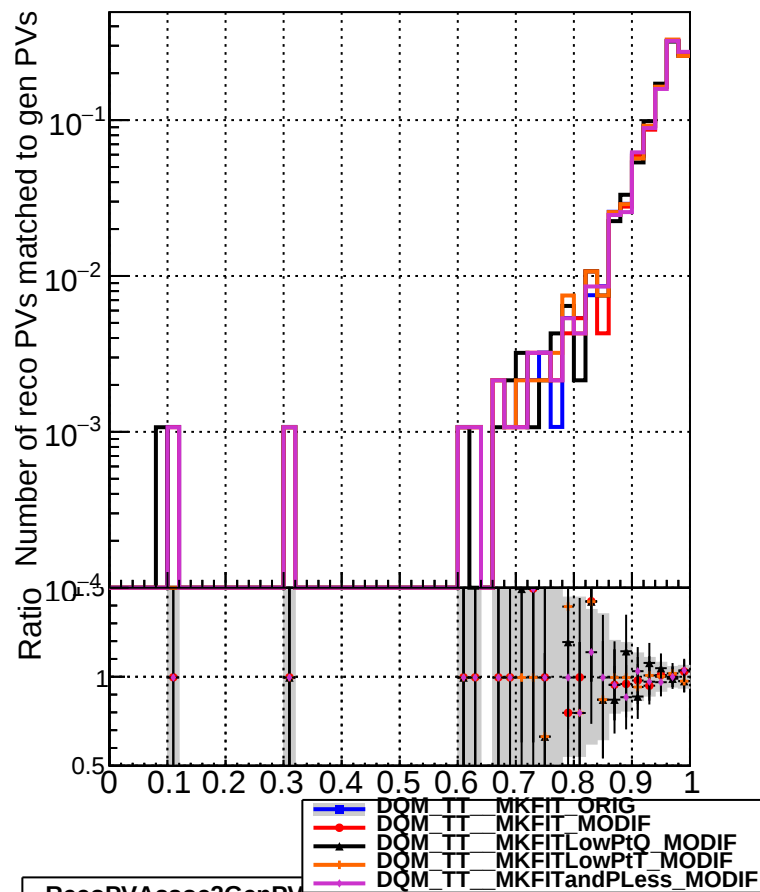
RecoPVAssoc2GenPVmatched_missing
