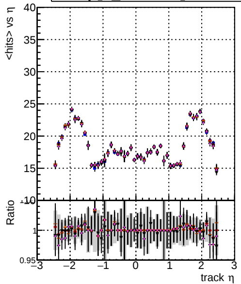
mean hits vs \eta DOM TT MKFIT ORIG DOM TT MKFIT MODIF DOM TT MKFITLowPIT MODIF DOM TT MKFITandPIT MODIF
