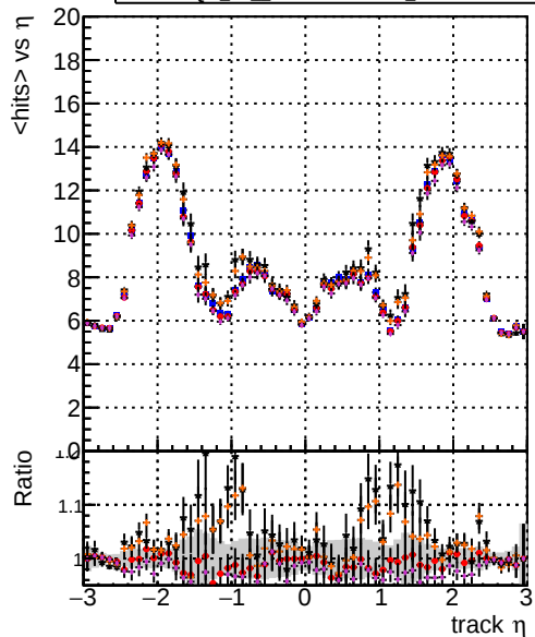
mean hit DOM TT MKFIT ORIS DOM TT MKFIT MODIF DOM TT MKFITLowPRO MODIF DOM TT MKFITLowPIT MODIF DOM TT MKFITandPless MODIF
