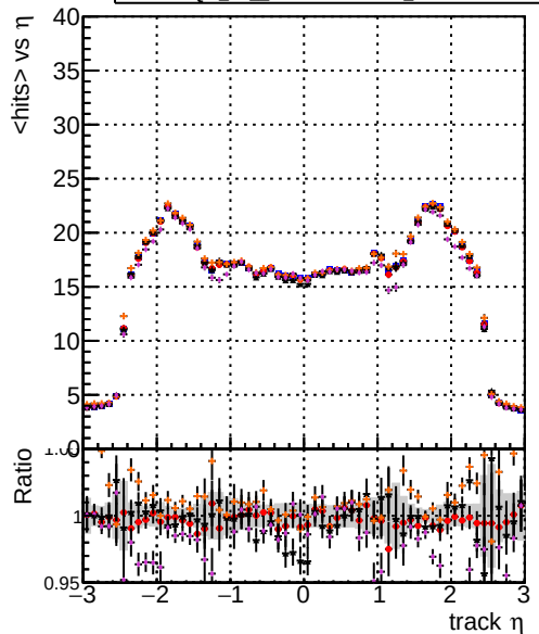
Legend for mean hits vs \eta : DOM TT MKFIT ORIG DOM TT MKFIT MODIF DOM TT MKFITLowPIT MODIF DOM TT MKFITLowPIT MODIF DOM TT MKFITandPless MODIF
