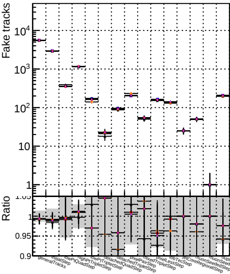
Number Symbol Variable ▲ DQM_TT_MKFITLowPto_MODIF ● DQM_TT_MKFITLowPtt_MODIF ▼ DQM_TT_MKFITandPLess_MODIF
