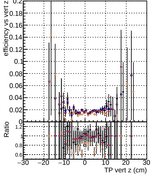
Efficiency vs. TP vert z DOM TT MKFIT ORIS DOM TT MKFIT MODIF DOM TT MKFITLowPIT MODIF DOM TT MKFITandPless MODIF
