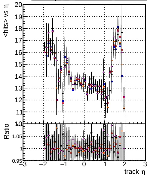
mean hits DOM TT MKFIT ORIG DOM TT MKFIT MODIF DOM TT MKFITLowPT MODIF DOM TT MKFITandPless MODIF
