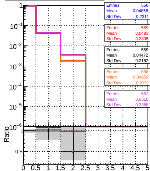
mean hits vs \eta Legend: DOM TT MKFIT ORIG DOM TT MKFIT MODIF DOM TT MKFITLowPIT MODIF DOM TT MKFITandPless MODIF
