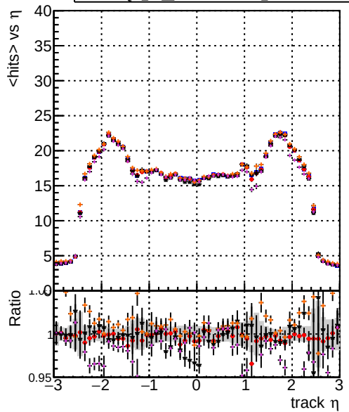
mean hits vs \eta DOM TT MKFIT ORIG DOM TT MKFIT MODIF DOM TT MKFITLowPIT MODIF DOM TT MKFITLowPIT MODIF DOM TT MKFITandPless MODIF
