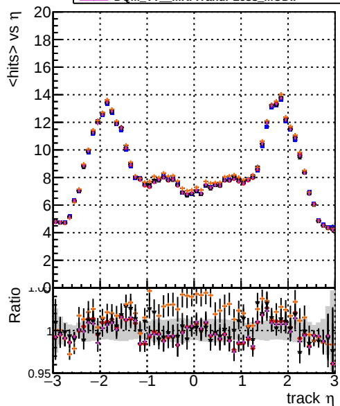
mean hits vs \eta DOM TT MKFIT ORIG DOM TT MKFIT MODIF DOM TT MKFITLowPIT MODIF DOM TT MKFITandPIT MODIF
