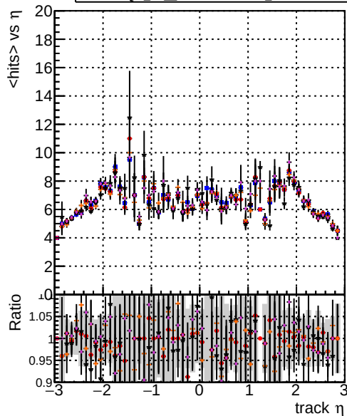
mean hit DOM TT MKFIT ORIS DOM TT MKFIT MODIF DOM TT MKFITLowPRO MODIF DOM TT MKFITLowPIT MODIF DOM TT MKFITandPless MODIF
