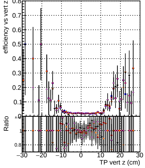
Efficiency vs vert z DOM TT MKFit ORIG DOM TT MKFit MODIF DOM TT MKFitLowPIT MODIF DOM TT MKFitandPless MODIF
