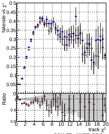
Fake rate vs. DOM IT MKFIT ORIG ACES DOM IT MKFIT and Less MODIF
