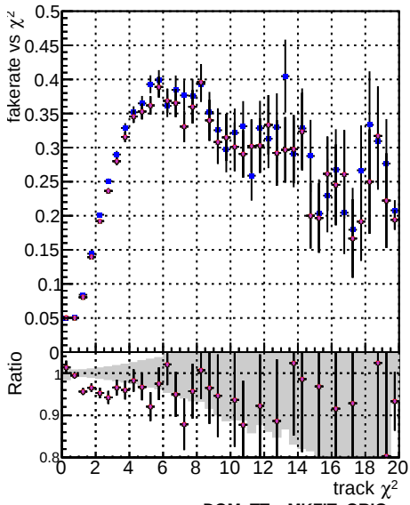
Fake rate vs. DOM IT MKFIT ORIG RACKS DOM IT MKFIT and Less MODIF
