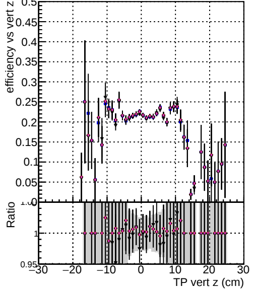
Efficiency vs. sim PV z — DOM TT MKFIT ORIS — DOM TT MKFIT MODIF — DOM TT MKFITLowPIT MODIF — DOM TT MKFITLowPIT MODIF — DOM TT MKFITandPless MODIF
