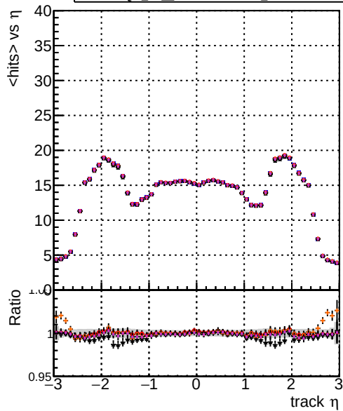
mean hit DOM TT MKFIT ORIG DOM TT MKFIT MODIF DOM TT MKFITLowPT MODIF DOM TT MKFITandPit MODIF DOM TT MKFITandPit MODIF
