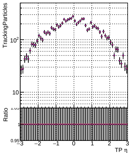
N of sim Model Model Model Model 1 DOM TT MKFITLowPto MODIF 2 DOM TT MKFITLowPtt MODIF 3 DOM TT MKFITandPless MODIF
