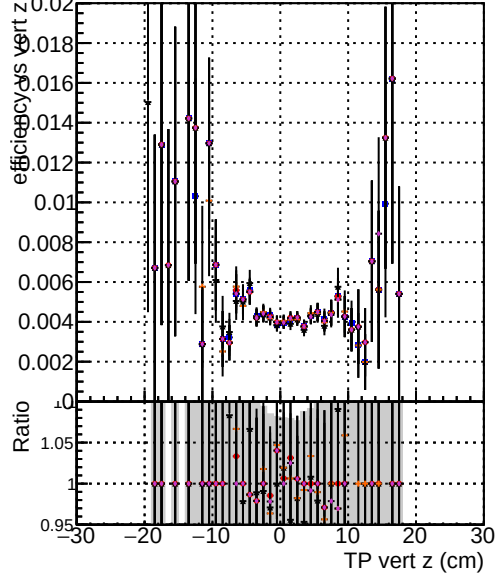
Efficiency vs. TP vert z (cm) DOM TT MKFIT ORIS DOM TT MKFIT MODIF DOM TT MKFITLowPIT MODIF DOM TT MKFITandPless MODIF
