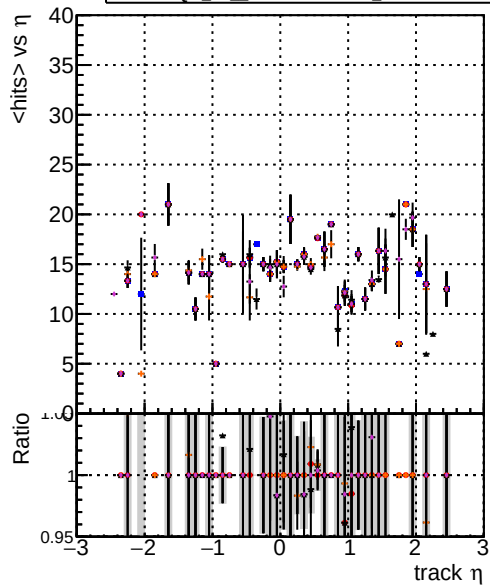
mean hits vs \eta DOM TT MKFIT ORIS DOM TT MKFIT MODIF DOM TT MKFITLowPIT MODIF DOM TT MKFITandPless MODIF
