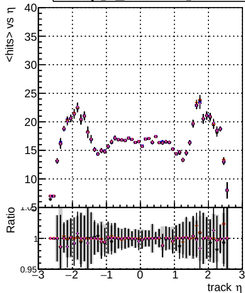
mean hits DOM TT MKFIT ORIS DOM TT MKFIT MODIF DOM TT MKFITLowPIT MODIF DOM TT MKFITandPless MODIF
