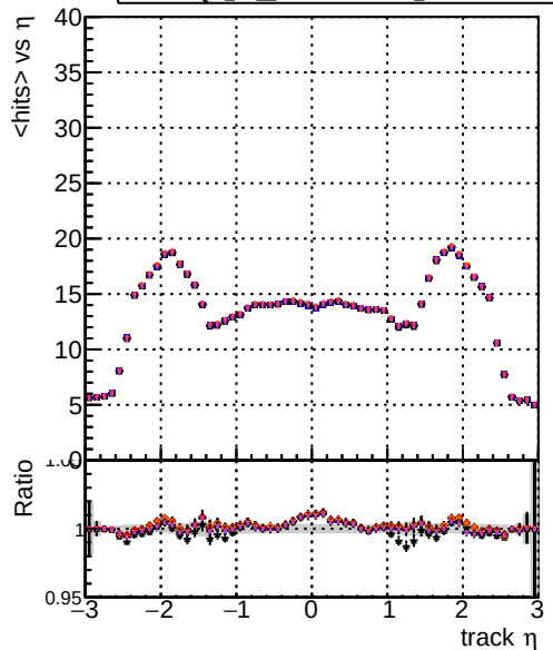
mean hits vs \eta DOM TT MKFIT ORIG DOM TT MKFIT MODIF DOM TT MKFITLowPIT MODIF DOM TT MKFITandPless MODIF
