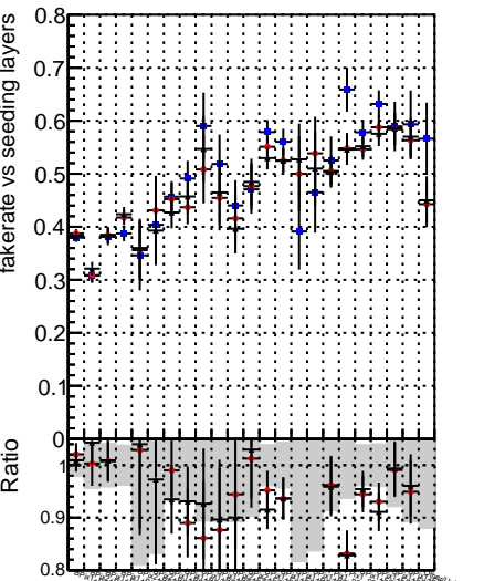
Fake rate vs. —●— DGM TT CKF ORIG —●— DGM TT CKF LOWPIT ORIG —●— DGM TT CKF LOWPIT MODIF
