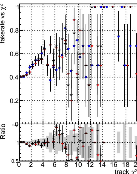
Fake rate vs. —●— DGM TT CKF ORIG —●— DGM TT CKF LOWPIT ORIG —●— DGM TT CKF LOWPIT MODIF
