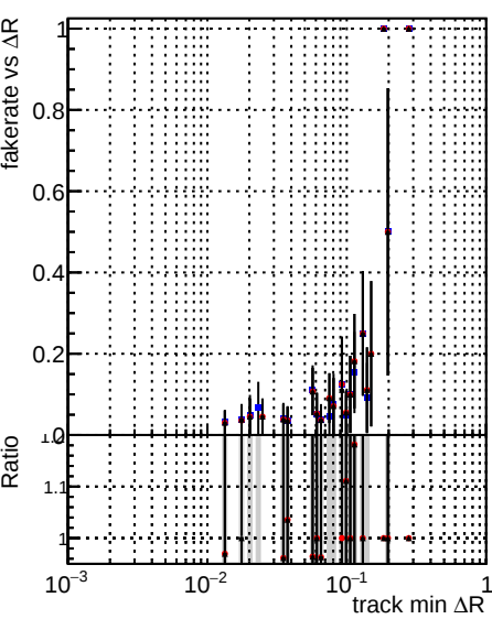
Fake rate vs \Delta R(\text{track}, \text{jet}) DOM TT CKF ORIG DOM TT CKF LOW Pt ORIG DOM TT CKF LOW Pt MODIF
