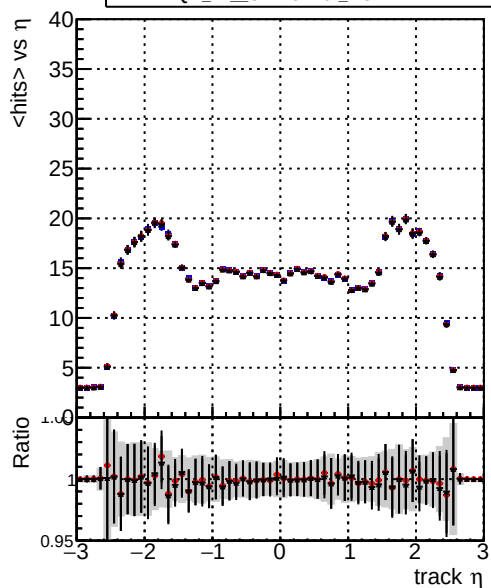
mean hit Legend: DQM_TT_CKF_ORIG (blue), DQM_TT_CKFlowPIT_ORIG (red), DQM_TT_CKFlowPIT_MODIF (black)
