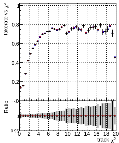
Fake rate vs. Legend DOM TT CKF ORIG DOM TT CKF LOWPIT ORIG CKF LOWPIT MODIF Line Blue Red Black Black Black Black Point Blue Red Black Black Black Black
