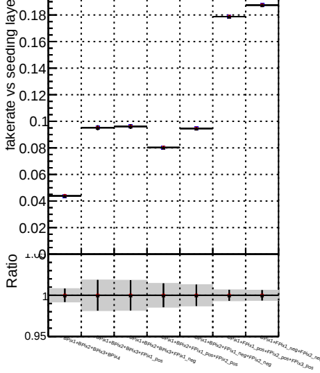
Fake rate vs seeding layers
