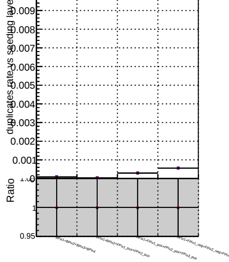
Duplicates Rate vs seeding layers
