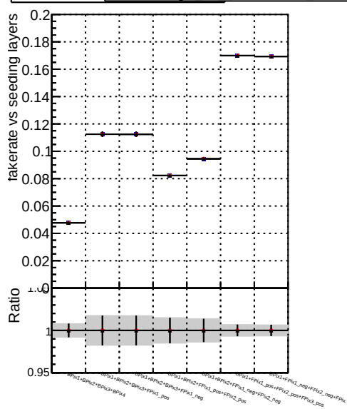
Fake rate vs. DOM TT CKF ORIG DOM TT CKF LOWPIT ORIG DOM TT CKF LOWPIT MODIF
