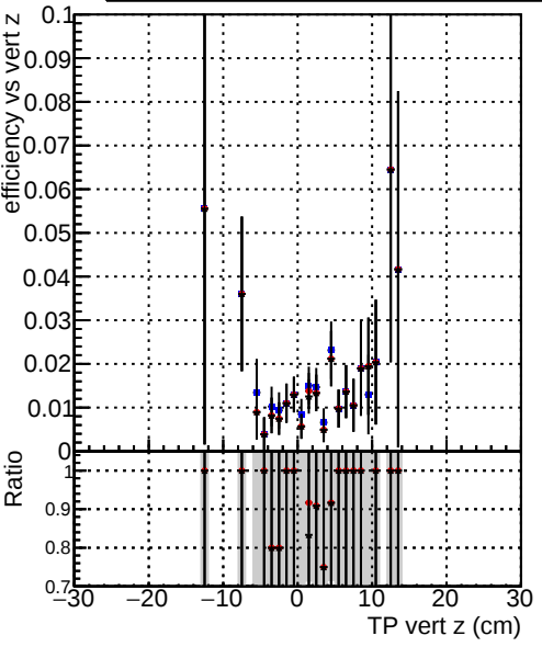
Efficiency vs TP vert z (cm) Legend: DQM_TT_CKF_ORIG (Blue diamonds) DQM_TT_CKFlowPtT_ORIG (Red circles) DQM_TT_CKFlowPtT_MODIF (Black triangles)
