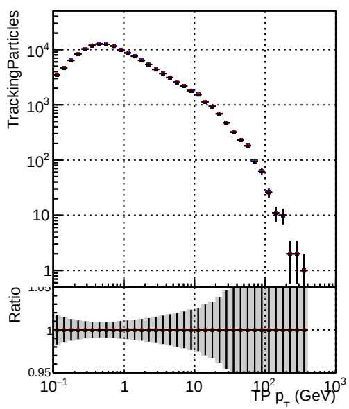
Legend: - DQM_TT_CKF_ORIG (blue circles) - DQM_TT_CKFlowPIT_ORIG (red circles) - DQM_TT_CKFlowPIT_MODIF (black circles) N of simulated tracks
