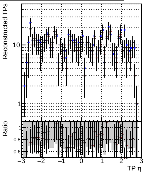
Legend: - DQM_TT_CKF_ORIG (blue circles) - DQM_TT_CKFlowPIT_ORIG (red circles) - DQM_TT_CKFlowPIT_MODIF (black circles) N of simulated tracks
