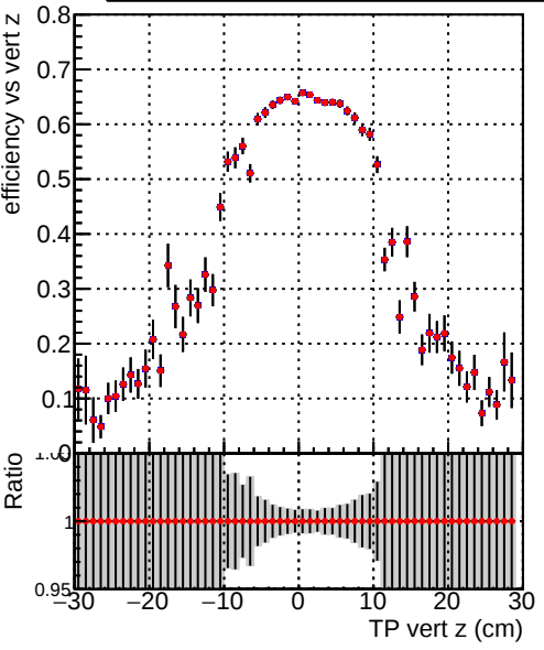
Efficiency vs TP vert z (cm) Legend: DQM_TT_CKF_ORIG (blue squares), DQM_TT_CKF_MODIF (red diamonds)
