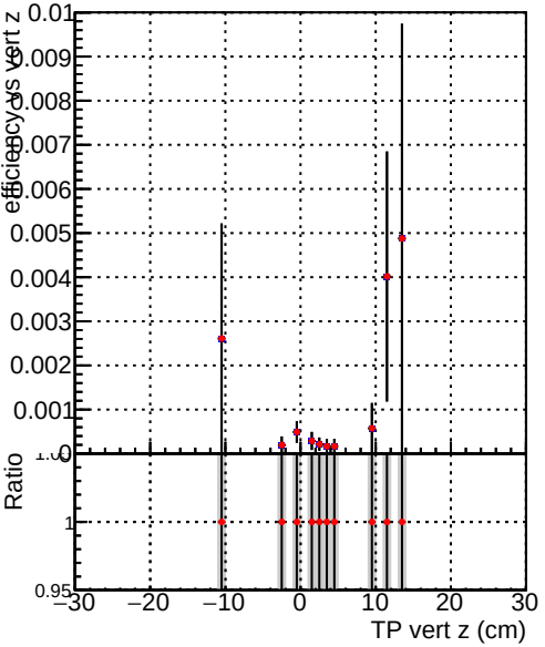
Efficiency vs vertpos Legend: DQM_TT_CKF_ORIG DQM_TT_CKF_MODIF
