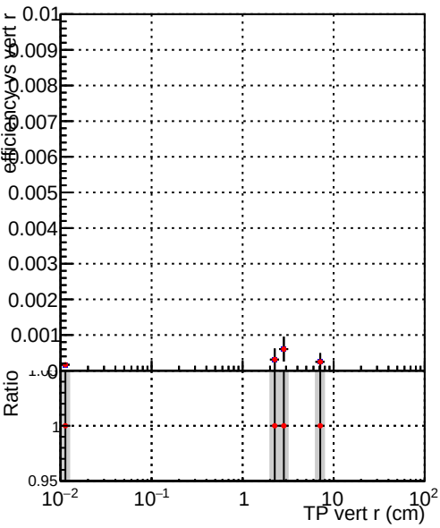
Efficiency vs vertpos Legend: DQM_TT_CKF_ORIG DQM_TT_CKF_MODIF
