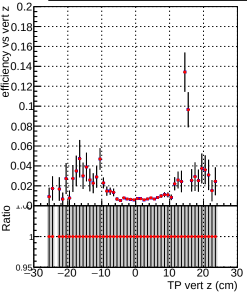
Efficiency vs TP vert z (cm) Legend: DQM_TT_CKF_ORIG (grey bars) DQM_TT_CKF_MODIF (red line with error bars)
