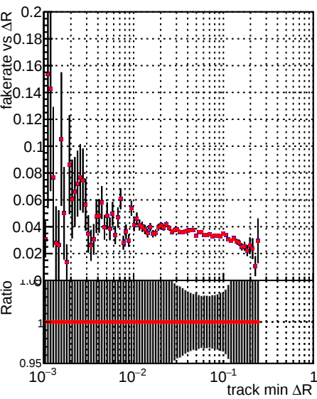
Fake rate vs \Delta R(\text{track}, \text{jet}) Legend: \Delta R(\text{track}, \text{jet}) (black line with error bars) \Delta R(\text{track}, \text{jet}) (red line with error bars)
