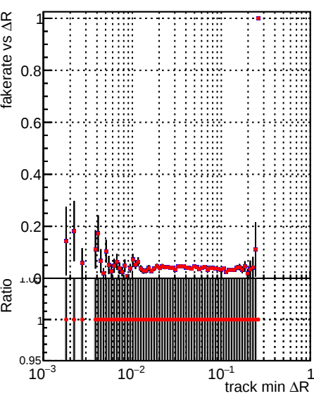
Fake rate vs \Delta R(\text{track}, \text{jet}) Legend: \Delta R(\text{track}, \text{jet}) (grey line with dots) \Delta R(\text{track}, \text{jet}) (red line with dots)
