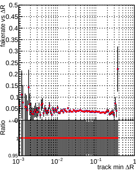
Fake rate vs \Delta R(\text{track}, \text{jet}) Legend: \blacksquare DQM_TT_CKF_ORIG \bullet DQM_TT_CKF_MODIF
