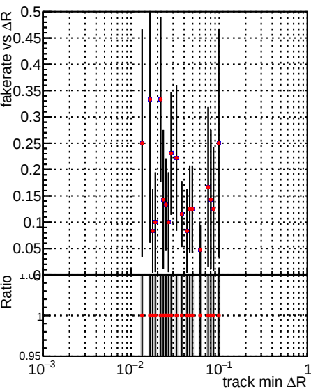
Fake rate vs ΔR(track, jet) DQM_TT_CKF_ORIG DQM_TT_CKF_MODIF
