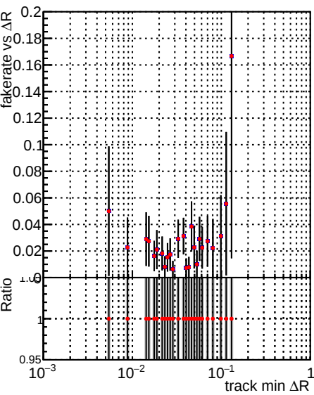
Fake rate vs \Delta R(\text{track, jet}) Legend: \Delta R(\text{track, jet}) (black line with dots) \Delta R(\text{track, jet}) (red line with dots)
