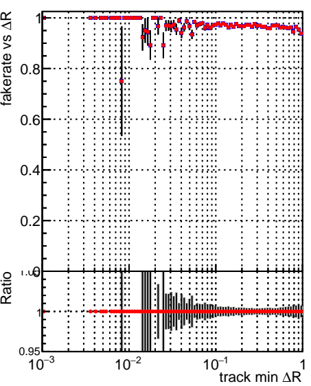
Fake rate vs \Delta R (track, jet) —●— DQM_TT_CKF_ORIG —●— DQM_TT_CKF_MODIF
