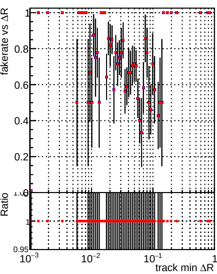
Fake rate vs \Delta R(\text{track, jet}) Legend: \blacksquare DQM_TT_CKF_ORIG \bullet DQM_TT_CKF_MODIF
