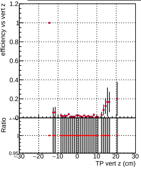
Efficiency vs TP vert z (cm) Legend: DQM_TT_CKF_ORIG (grey bar) DQM_TT_CKF_MODIF (red line)
