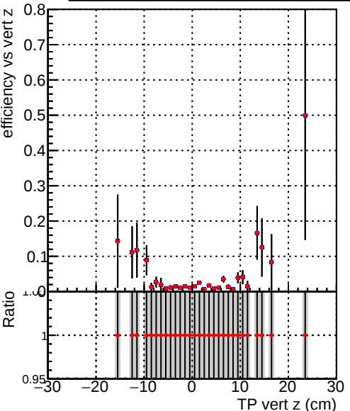
Efficiency vs TP vert z (cm) Legend: DQM_TT_CKF_ORIG (grey histogram) DQM_TT_CKF_MODIF (red dots with error bars)
