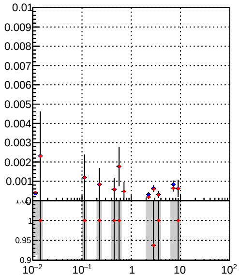
Efficiency vs vertpos Legend: — * /data2/legianni/BDT-vs-DNN/real-BDT/CMSSW_13_0_0_pre4/src/runrem/DQM_TT_mkFit_ — * DQM_TT_mkFit_
