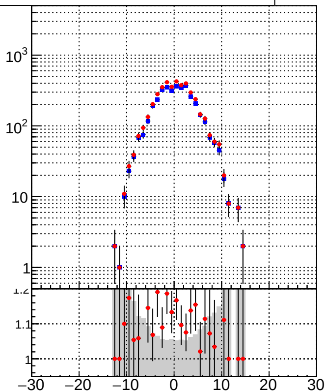
/data2/legianni/BDT-vs-DNN/real-BDT/CMSSW_13_0_0_pre4/src/runrem/DQM_TT_mkFit_
