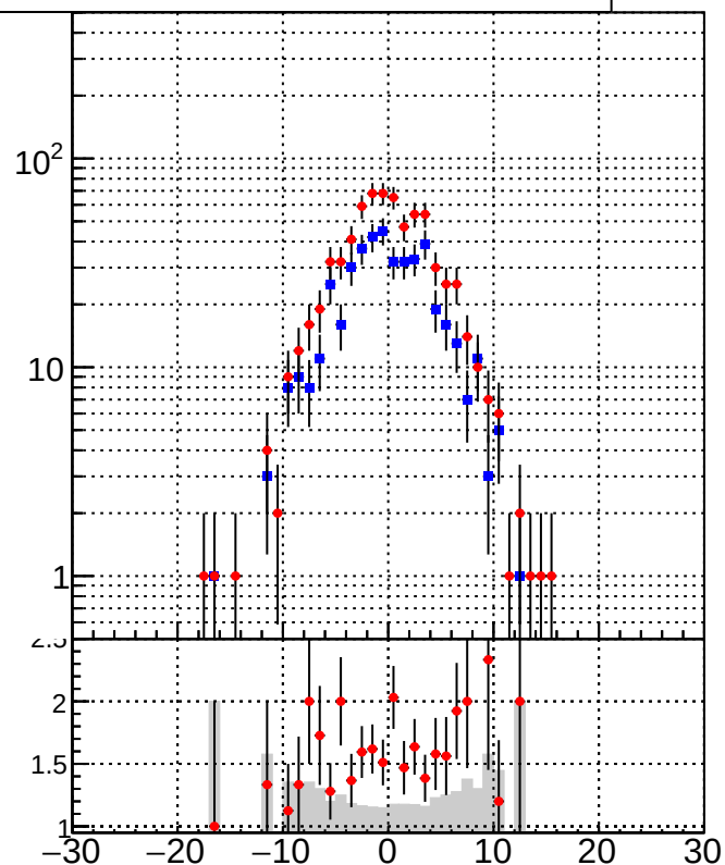
■ /data2/legianni/BDT-vs-DNN/real-BDT/CMSSW_13_0_0_pre4/src/runrem/DQM_TT_mkFit_ ■ DQM_TT_mkFit_
