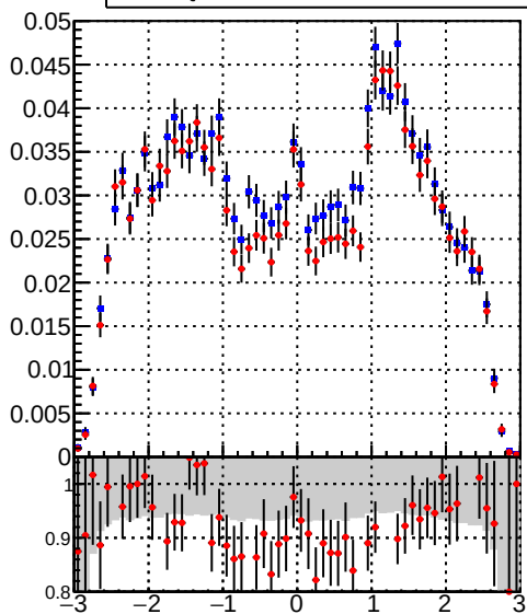
/data2/legianni/BDT-vs-DNN/real-BDT/CMSSW_13_0_0_pre4/src/runrem/DQM_TT_mkFit_ DQM_TT_mkFit_
