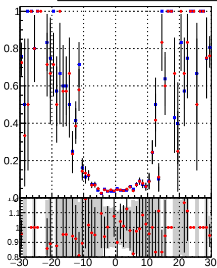
Legend: - Blue line with markers: /data2/legianni/BDT-vs-DNN/real-BDT/CMSSW_13_0_0_pre4/src/runrem/DQM_TT_mkFit_ - Red line with markers: DQM_TT_mkFit_ - Grey histogram: (unlabeled)
