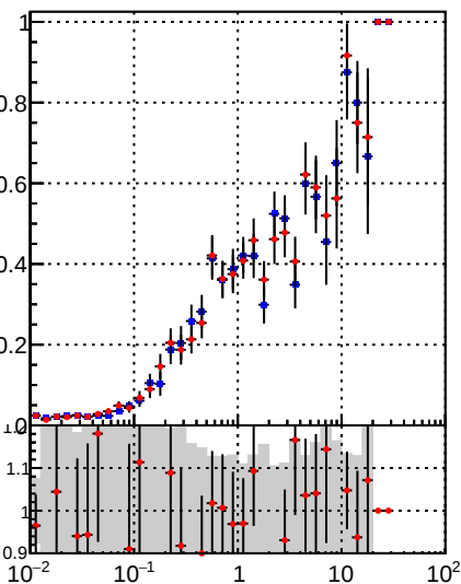
Legend: - Blue line with markers: /data2/legianni/BDT-vs-DNN/real-BDT/CMSSW_13_0_0_pre4/src/runrem/DQM_TT_mkFit_ - Red line with markers: DQM_TT_mkFit_ - Grey histogram: (unlabeled)
