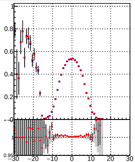
/data2/legianni/BDT-vs-DNN/real-BDT/CMSSW_13_0_0_pre4/src/runrem/DQM_TT_mkFit_ DQM_TT_mkFit_
